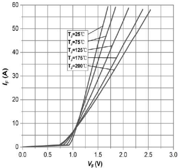
Figure 1: Forward Characteristics
