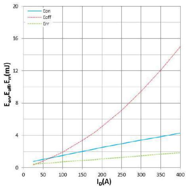
Figure 14. E on , E off , E rr vs I DS
