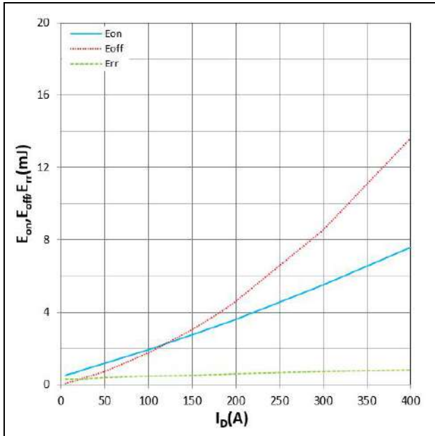
Figure 13. E on , E off , E rr vs I DS
