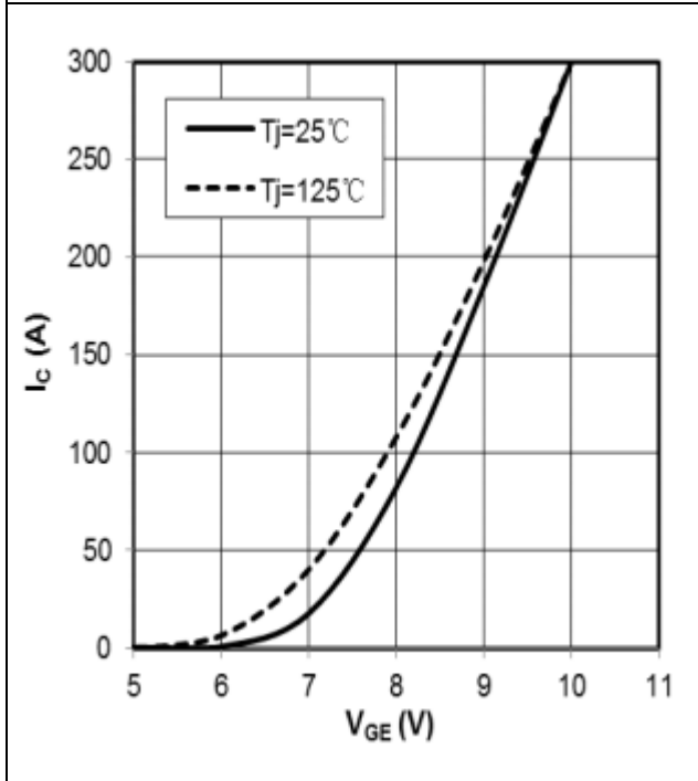
Figure 7. I_c vs V_{GE} V_{CE}=20V
