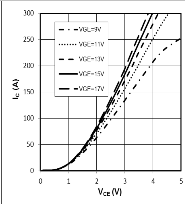
Figure 6. I_c vs V_{CE} T_j=125^\circ C
