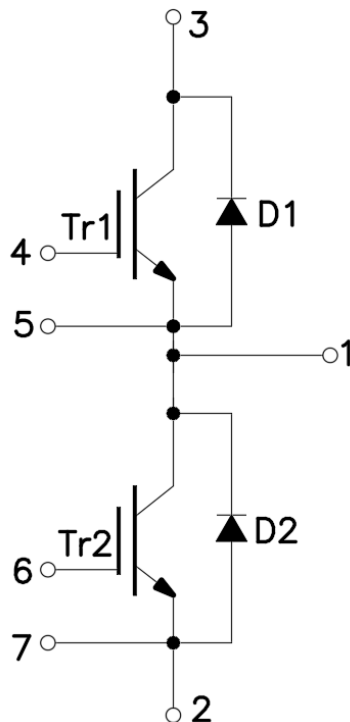
Figure 1. Out drawing & circuit diagram for HCG150FF120A11
