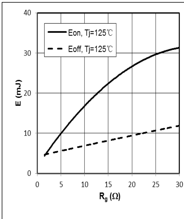
Figure 9. E_{on} , E_{off} vs R_g (Typ) V_{CC}=600V , V_{GE}=+15V/-15V , I_C=150A
