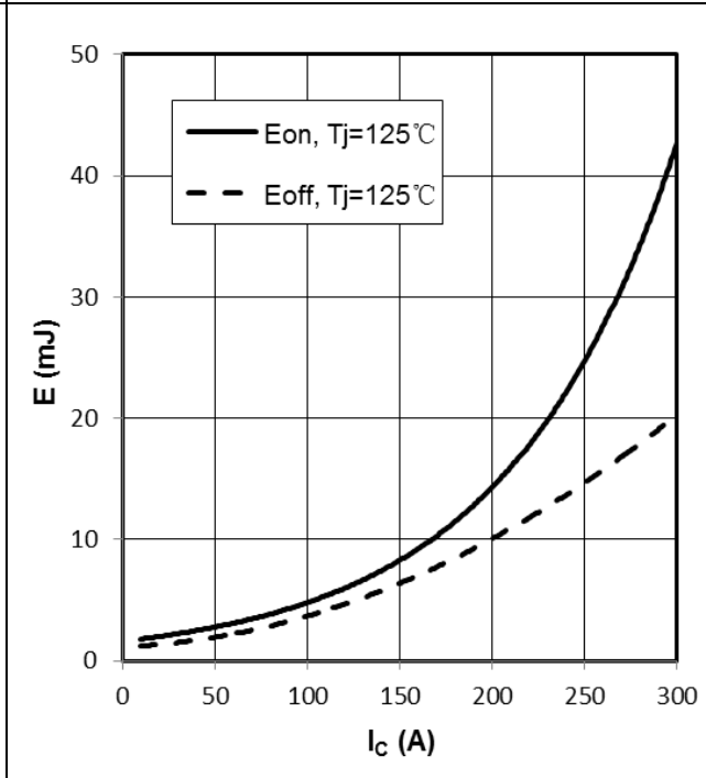
Figure 8. E_{on}, E_{off} vs I_c (Typ) V_{CC}=600V, V_{GE}=+15V/-15V, R_G=4.7\Omega
