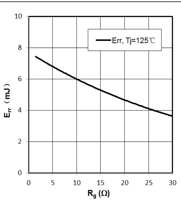
Figure 14. Switching losses Diode, E_{rr}=f(R_g) , I_F=150A , V_{CE}=600V
