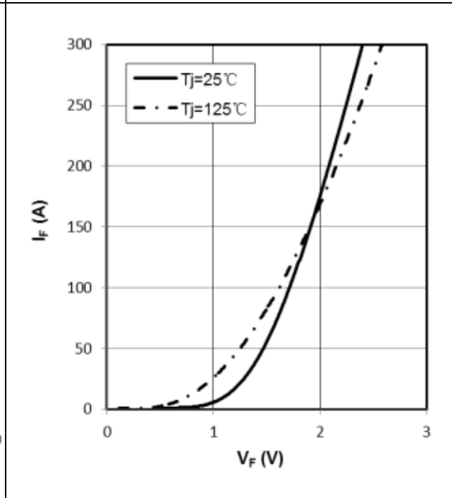
Figure 12. Forward characteristic of Diode , I_F=f(V_F)
