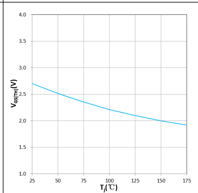
Figure 12. V_{GS(TH)} vs T_j V_{GS}=V_{DS}, I_D=300mA
