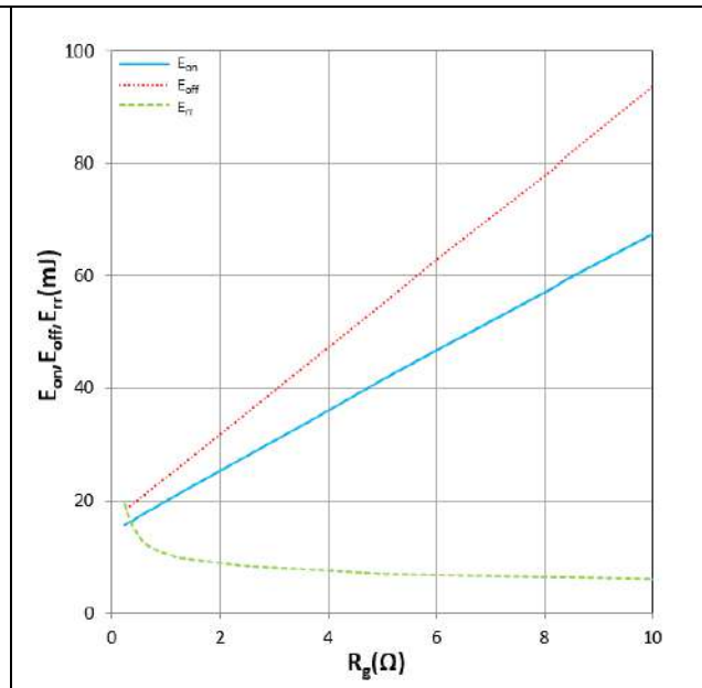
Figure 14. E_{on} , E_{off} , E_{rr} vs R_g
