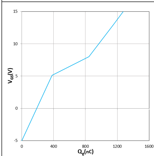
Figure 11. V_{GS} vs Q_g T_j=25^\circ C, V_{DS}=1000V, I_D=375A
