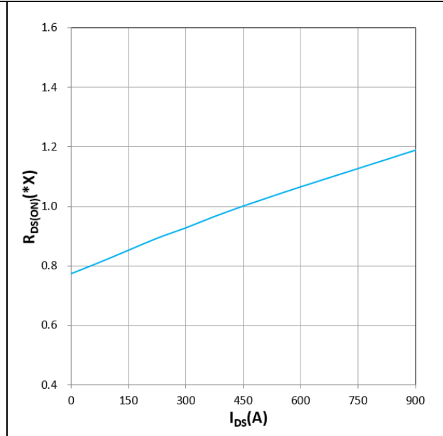
Figure 10. R_{DS(ON)} vs I_{DS} T_j=25^\circ C, V_{GS}=+15V, 1.0X=4.3m\Omega
