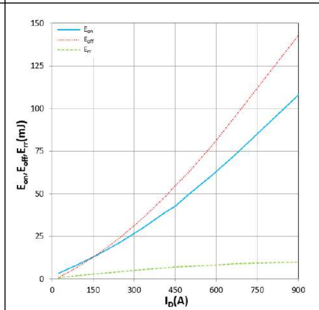
Figure 16. E_{on} , E_{off} , E_{rr} vs I_D
