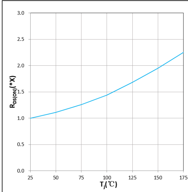
Figure 9. R_{DS(ON)} vs T_j V_{GS}=+15V, I_D=600A, 1.0X=4.3m\Omega
