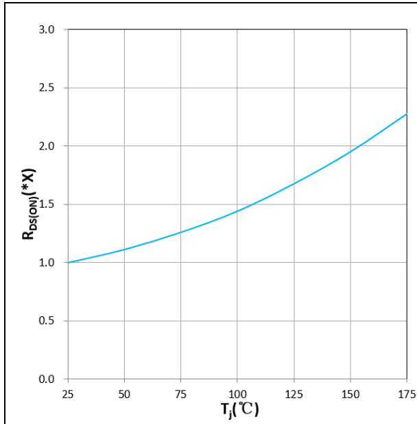
Figure 9. R_{DS(ON)} vs T_j V_{GS} = +15V , I_D = 600A , 1.0X = 3.4m\Omega
