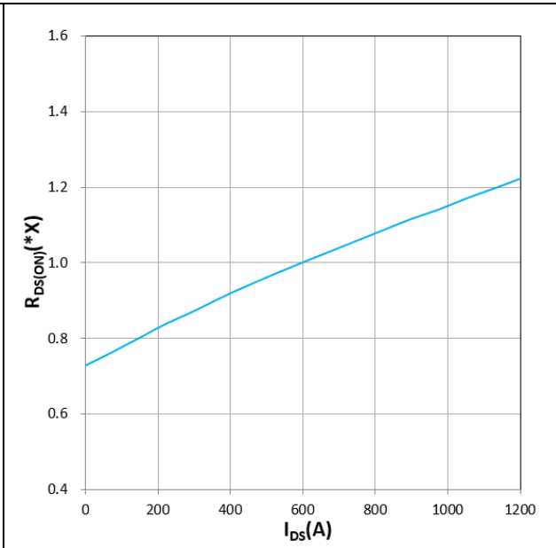
Figure 10. R_{DS(ON)} vs I_{DS} T_j = 25^\circ C , V_{GS} = +15V , 1.0X = 3.4m\Omega
