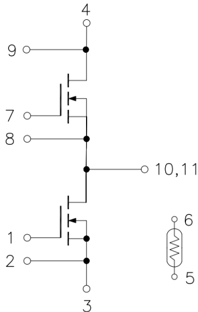
Figure 1. Out drawing & circuit diagram for HCS600FF220E3T1
