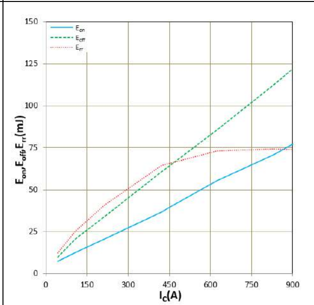
Figure 14. E on , E off , E rr vs I c (Typ) V CC =600V, V GE =+15V/-8V, R g =1.3Ω, T j =150°C Inductive Load
