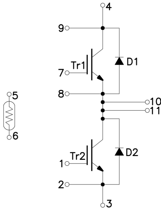
Figure 1. Out drawing & circuit diagram for HCG450FH120D3ME7
