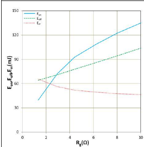
Figure 13. E on , E off , E rr vs R g (Typ) V CC =600V, V GE =+15V/-8V, I C =450A, T j =150°C Inductive Load
