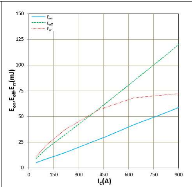
Figure 12. E on , E off , E rr vs I c (Typ) V CC =600V, V GE =+15V/-8V, R g =1.3Ω, T j =125°C Inductive Load
