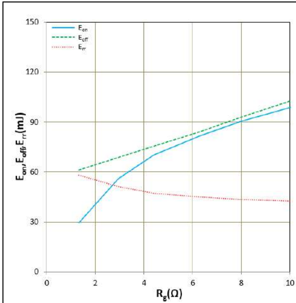
Figure 11. E on , E off , E rr vs R g (Typ) V CC =600V, V GE =+15V/-8V, I C =450A, T j =125°C Inductive Load
